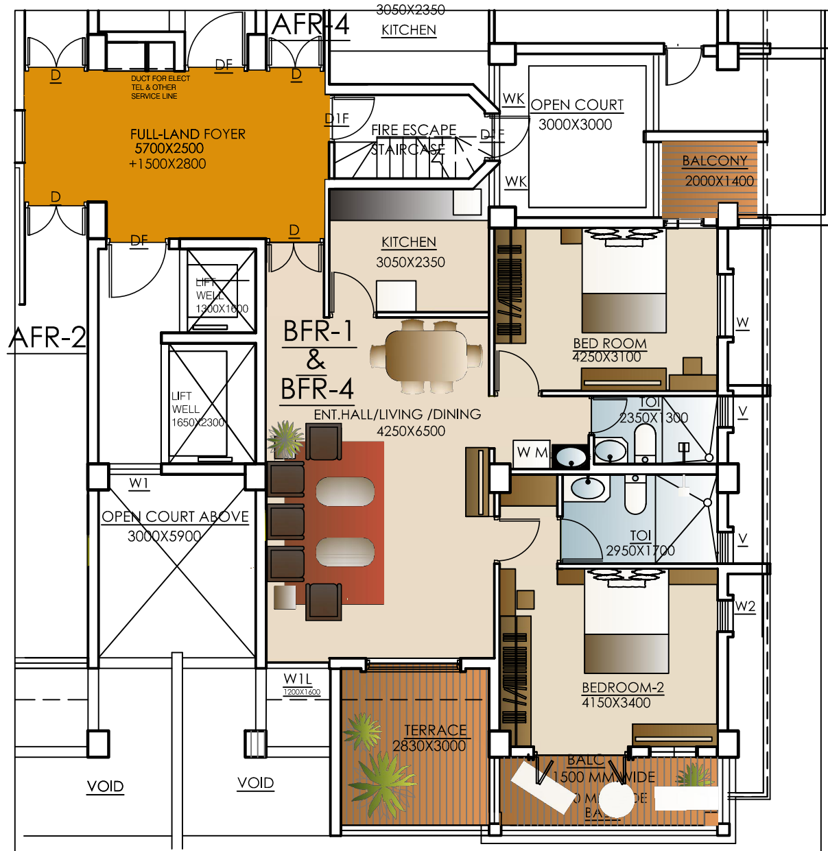
DETAIL OF FLAT 'FR1' & FR4 IN BLOCK 'B'
